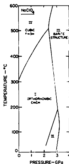
Fig. 4. High pressure phase diagram of \text{NaClO}_4 .
