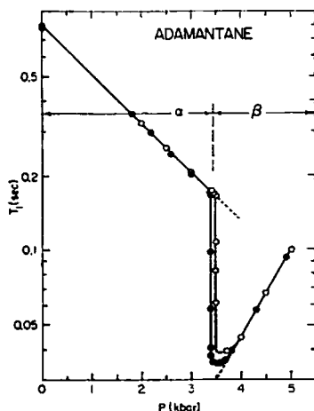
Fig. 7. Pressure dependence of the proton T_1 for adamantane dispersion in D_2O at 0^\circ C for compression ( \circ ) and decompression ( \bullet ) measurements. Dashed lines represent the linear extrapolation of T_1 into the phase transition region (Ref. 71).
