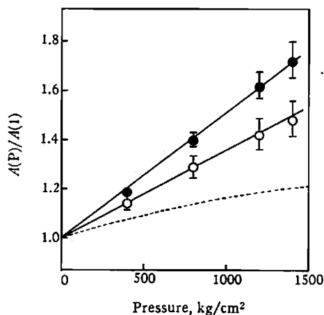
Fig. 3 Increase of the absorbance at absorption maximum as a function of pressure. The dotted line is the square of the relative density of solvent. ●: mesitylene-TCNE, ○: HMB-TCNE
