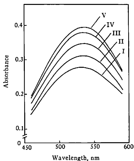
Fig. 2 Absorption spectra of HMB-TCNE complex in carbon tetrachloride at various pressures at 25°C (initial conc., HMB: 1.661 \times 10^{-2} mole/l, TCNE: 0.8096 \times 10^{-4} mole/l) I: 1 atm, II: 400 kg/cm 2 , III: 800 kg/cm 2 , IV: 1200 kg/cm 2 , V: 1400 kg/cm 2
