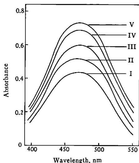
Fig. 1 Absorption spectra of mesitylene-TCNE complex in carbon tetrachloride at various pressures at 25°C. (initial conc., mesitylene: 5.051 \times 10^{-2} mole/l, TCNE: 4.886 \times 10^{-4} mole/l) I: 1 atm, II: 400 kg/cm 2 , III: 800 kg/cm 2 , IV: 1200 kg/cm 2 , V: 1400 kg/cm 2
