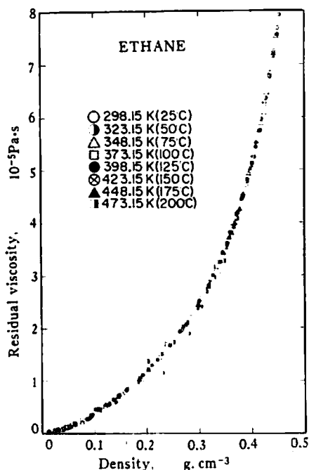
Fig. 5 Residual viscosity correlation for ethane
