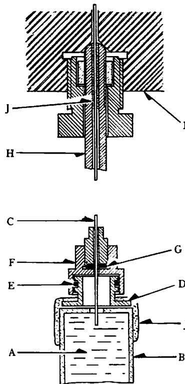
Fig. 2 Sampling system of high pressure apparatus
