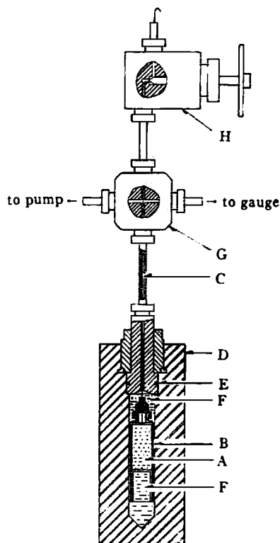
Fig. 1 High pressure apparatus for kinetic measurements
