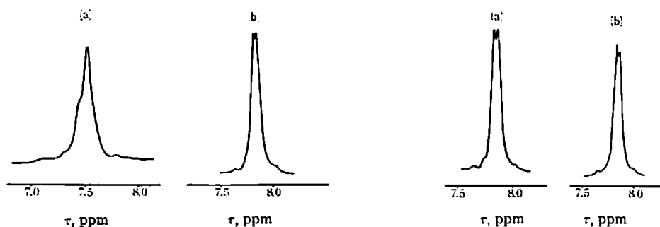
Fig. 2 Methylenic proton resonance of PAN- d\alpha_1 at 60 Mc/sec (a) in NaCNS-D 2 O at 120°C (b) in CD 3 NO 2 -(CH 2 O) 2 CO at 150°C
