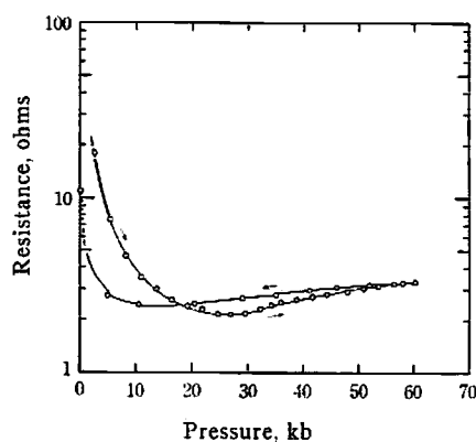
Fig. 7 Resistance versus pressure for CdO at room temperature
