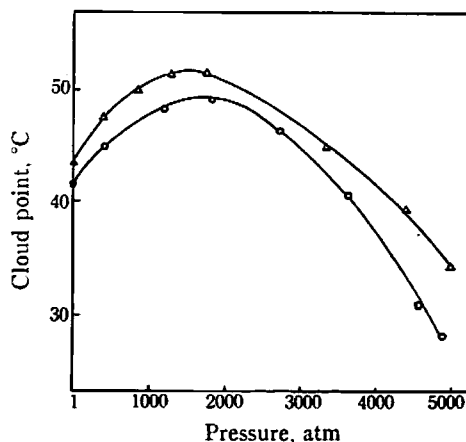
Fig. 4 Effect of pressure on the cloud point of polyoxyethylene nonylphenyl ether ( C_9H_{19}C_6H_4O(CH_2CH_2O)_{8.5}H —water —○—: 0.05 wt% —△—: 10.0 wt%
