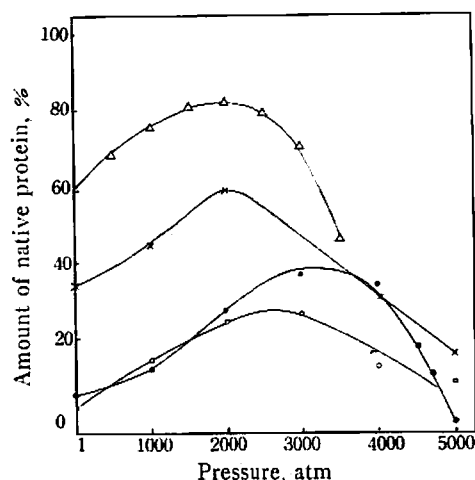
Fig. 2 Effect of pressure on heat denaturation of proteins (—x—, —●—) and effect of recompression on pressure denatured proteins (—Δ—, —○—)
