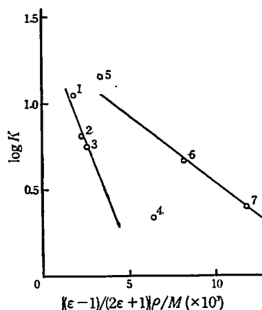
Fig. 7 Equilibrium constant of tautomerism for acetylacetone vs. solvent property \{(\epsilon-1)/(2\epsilon+1)\} \rho/M
