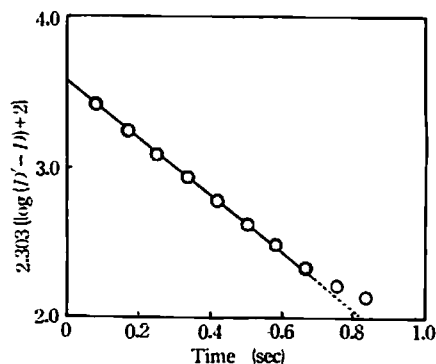
Fig. 4 Guggenheim's plot at 472 mμ
