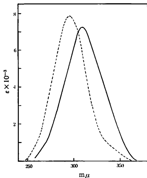
Fig. 11 Ultraviolet spectra of derivatives of neopentoylformoin in ethanol: mono-O-methyl neopentoylformoin (—); di-O-methyl neopentoylformoin (-----)
