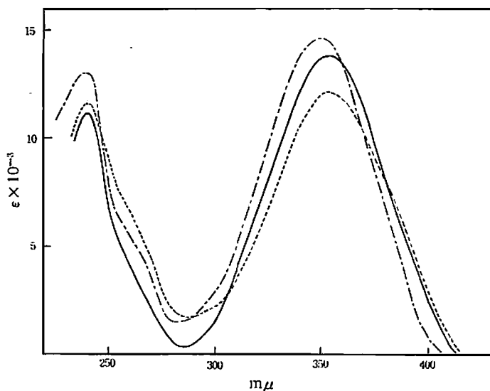
Fig. 9 Ultraviolet spectra of benzoylformoin in tetrahydrofuran (—), ether (---) and ethanol (.....)
