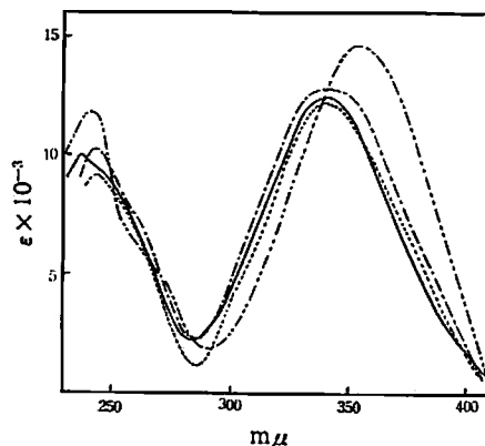
Fig. 12 Ultraviolet spectra of derivatives of benzoylformoin: 1st mono-O-methyl benzoylformoin in ethanol (---); di-O-methyl benzoylformoin in ethanol (-.-.-); 2nd mono-O-methyl benzoylformoin in tetrahydrofuran (—) and chloroform (.....)
