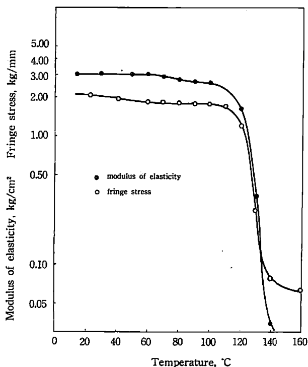
Fig. 4 Fringe stress and modulus of elasticity for the employed epoxy resin
