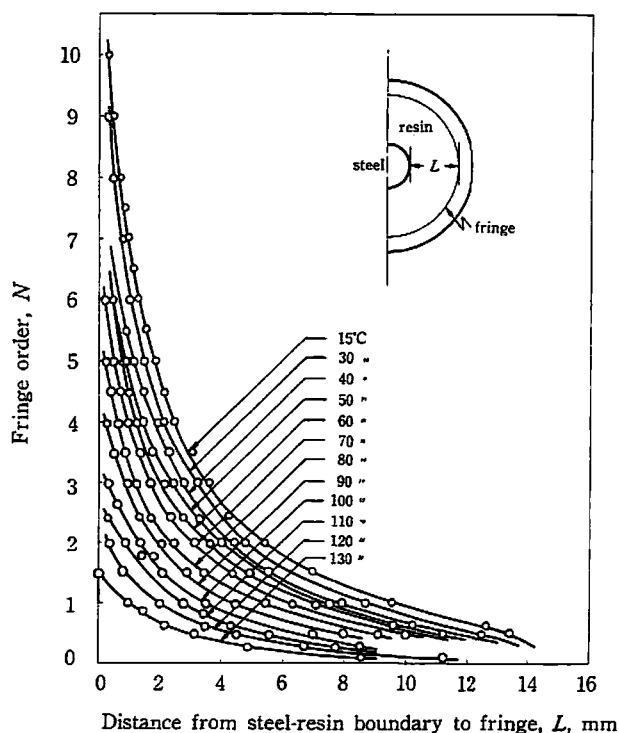
Fig. 3 Fringe-distribution in restrained model
