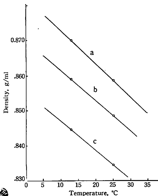
Fig. 1 Density of C_6H_6-CH_3OH system C_6H_6:CH_3OH (mole ratio)
