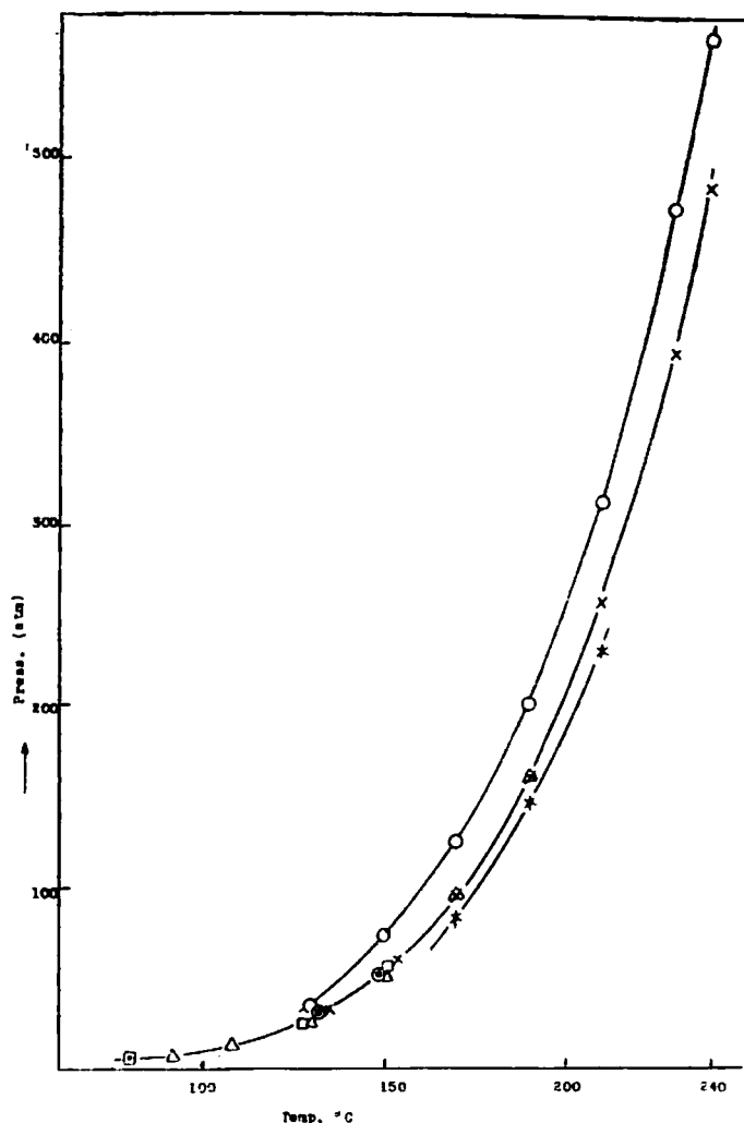
Fig. 2 Pressure—temperature curves.
