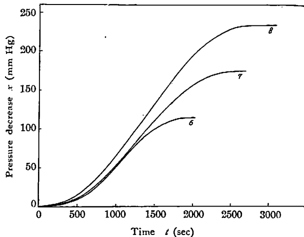
Fig. 5. Influence of initial pressure (at 180^\circ ).
