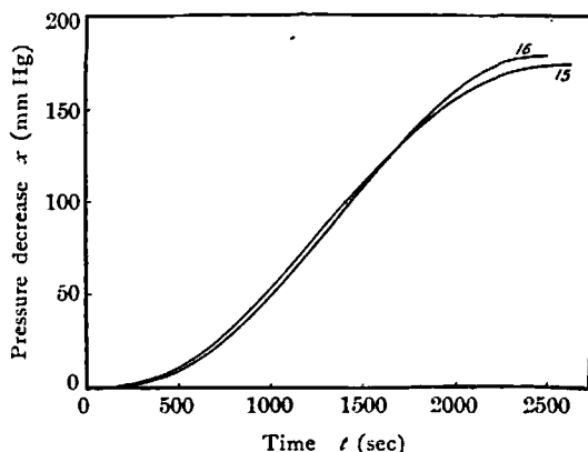
Fig. 11. Effect of water vapour (at 180°C).
