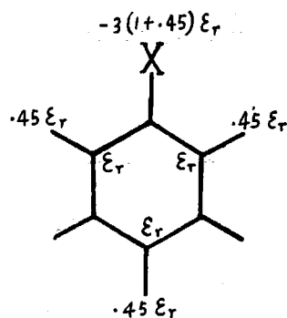
Fig. 3. Charge distribution due to inductive effect.
