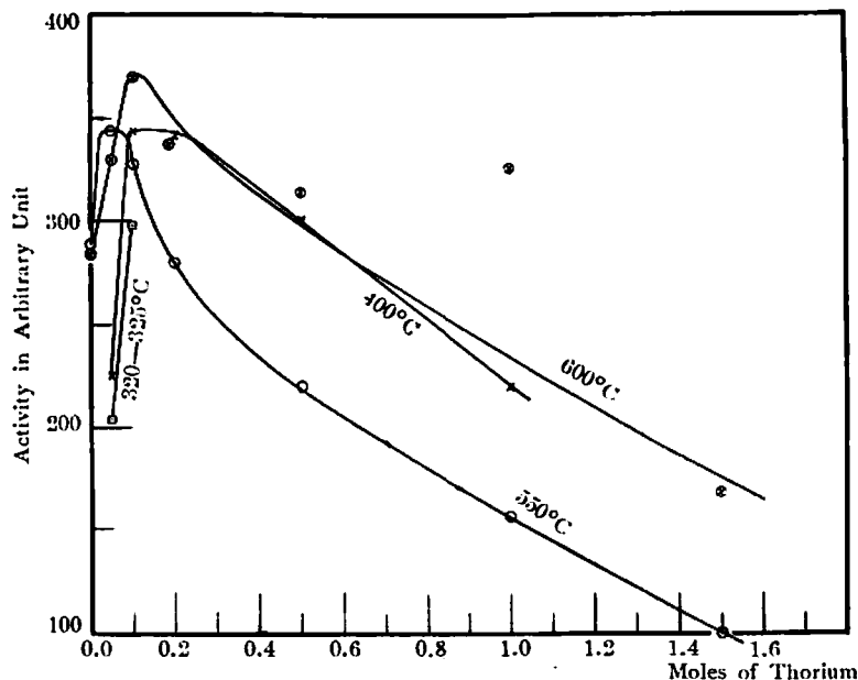
Fig. 1 Activity vs. Thorium Content (Reduction Temp ^\circ\text{C} are given)
