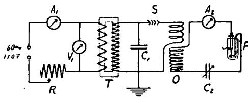
Fig. 2. Wiring diagram for high frequency current.
