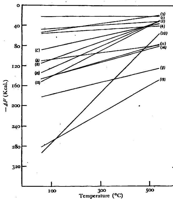
Fig. 1 \Delta F of Chain-Hydrocarbons.
