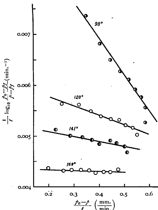
Fig. 5—The relation between \frac{1}{t} \log_{10} \frac{p_0 - p_f}{p - p_f} and \frac{p_0 - p}{t} . ( p_0 , initial pressure; p_f , final pressure; p , pressure at time t .)
