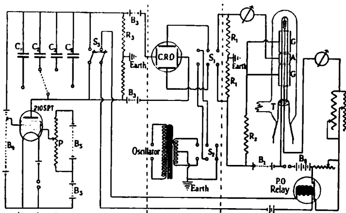
FIG. 1. C_1 0.5F. C_3 1F. C_3 2F. C_4 4F. R_1 10^3 to 10^4 ohms (strip). R_2 \frac{1}{2}R_1 . R_3 2 \times 10^4 ohms (strip). B_1 180 volts. B_2 8 volts, accumulator. 15 volts each. B_4 50 volts, auxiliary grid 80 volts. B_3 3 + 12 volts. P
