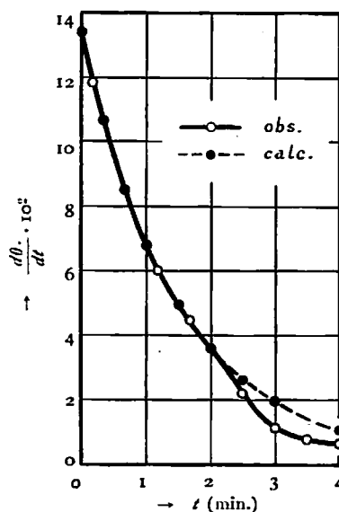
Fig. 12.—Expt. 12 (Pseudo-unimolecular).
