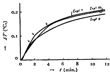
Fig. 8.—Salt effect.
