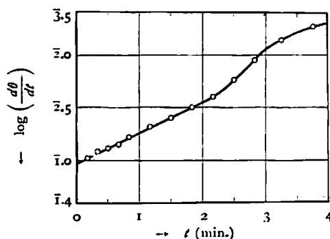
Fig. 11.—Expt. 12 (Pseudo-unimolecular).
