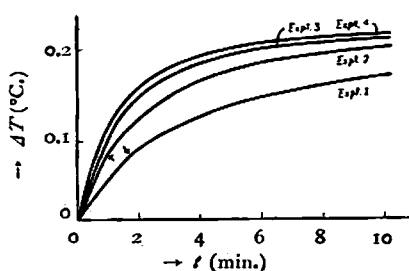
Fig. 2.—Influence of [II+].
