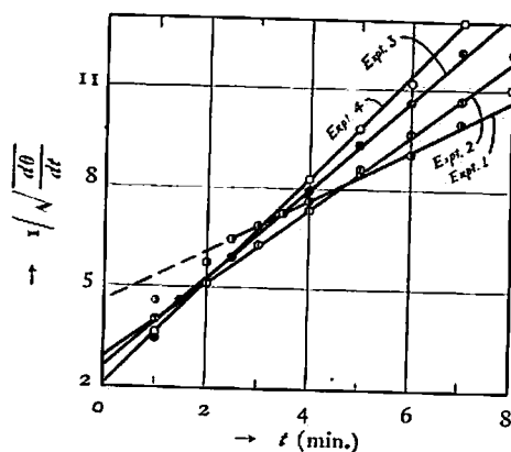
Fig. 4.—Influence of [H^+] .
