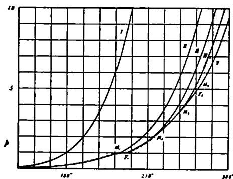
Fig. 4. Vapour Pressure of Concentrated aqueous Solution of \text{CaCl}_2 .
