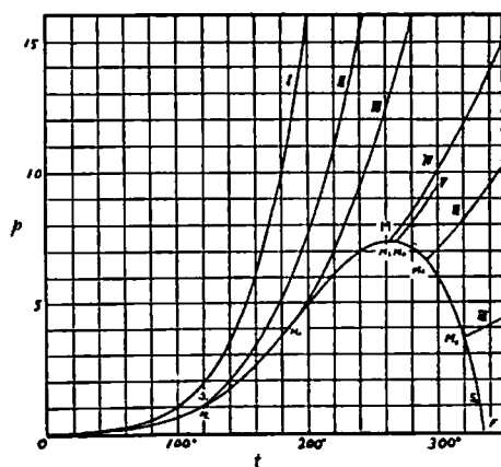
Fig. 3. Vapour Pressure of Concentrated aqueous Solution of \text{KNO}_3 .
