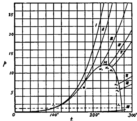
Fig. 1. Vapour Pressure of Concentrated aqueous Solution of \text{HgCl}_2 .
