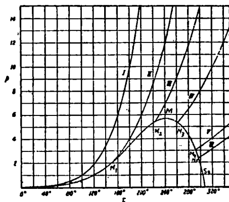
Fig. 2. Vapour Pressure of Concentrated aqueous Solution of \text{NaNO}_3 .
